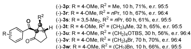
Scheme 4. Possible mechanistic pathway and control experiment. Qn = 8-methylquinoline.
