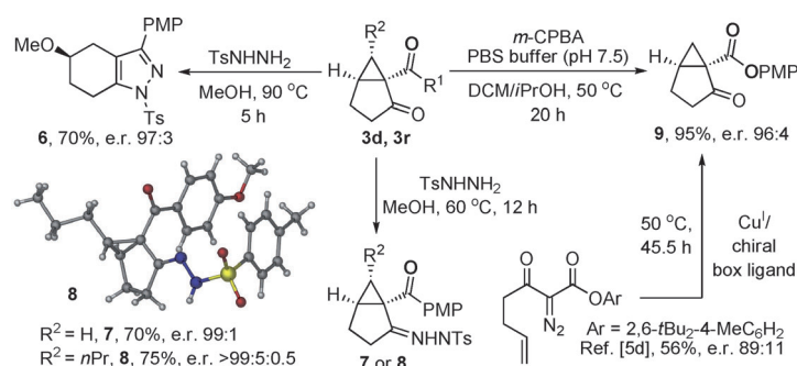
Scheme 5. Transformation of the product. box = bisoxazoline, m -CPBA = m -chloroperbenzoic acid, PBS = phosphate-buffered saline, Ts = p -toluenesulfonyl.
