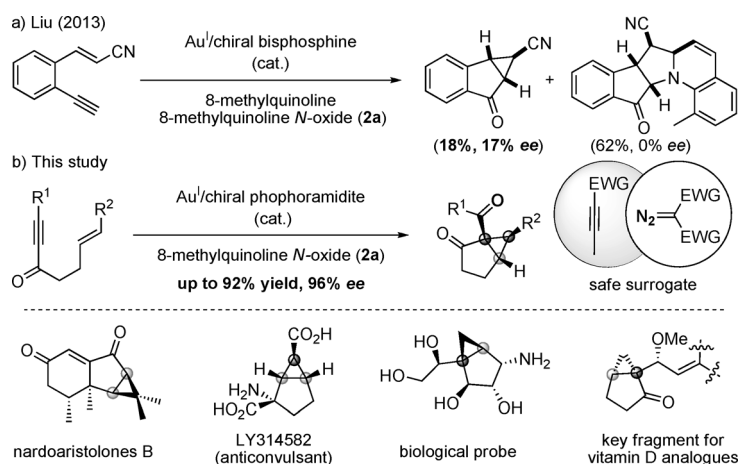
Scheme 1. Intramolecular cyclopropanation of enynes by gold(I)-catalyzed alkyne oxidation for the asymmetric synthesis of bicyclo[3.1.0]hexanes, and examples of compounds containing a bicyclo[3.1.0]hexane ring system. EWG = electron-withdrawing group.
