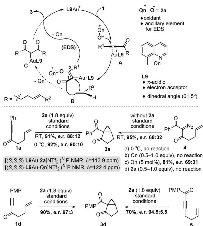
Scheme 4. Possible mechanistic pathway and control experiment. Qn = 8-methylquinoline.
