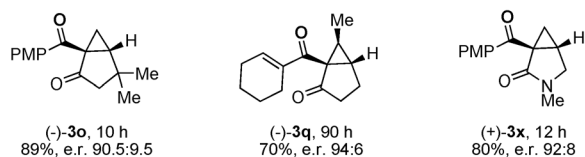
Scheme 3. Generality of the reaction. [a] The reaction was carried out with 1d (2.71 mmol) and [(S,S,S)-L9AuCl]/AgSbF 6 (4 mol %). [b] The diastereomeric ratio was determined by 1 H NMR spectroscopic and HPLC analysis. [c] The minor diastereomer was obtained with e.r. 85.5 : 14.5. PMP = 4-methoxyphenyl. Bn = benzyl, TBS = tert -butyldimethylsilyl.
